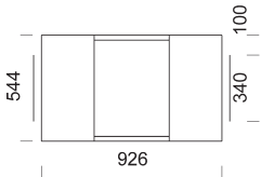
HESTIA SOLO 180 TUNNEL CERAMIC
